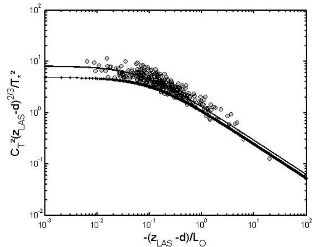
Fig. 2. Observed values of C_{T2}(z_{\text{LAS}} - d)^{2/3}/T_*^2 plotted against observed (z_{\text{LAS}} - d)/L_O during the 3 periods. Data that diverges from MOST behavior are rejected. Solid line represents the scaling of the universal function given by Hill (1992) and dotted line represents the one by de Bruin (1993).
