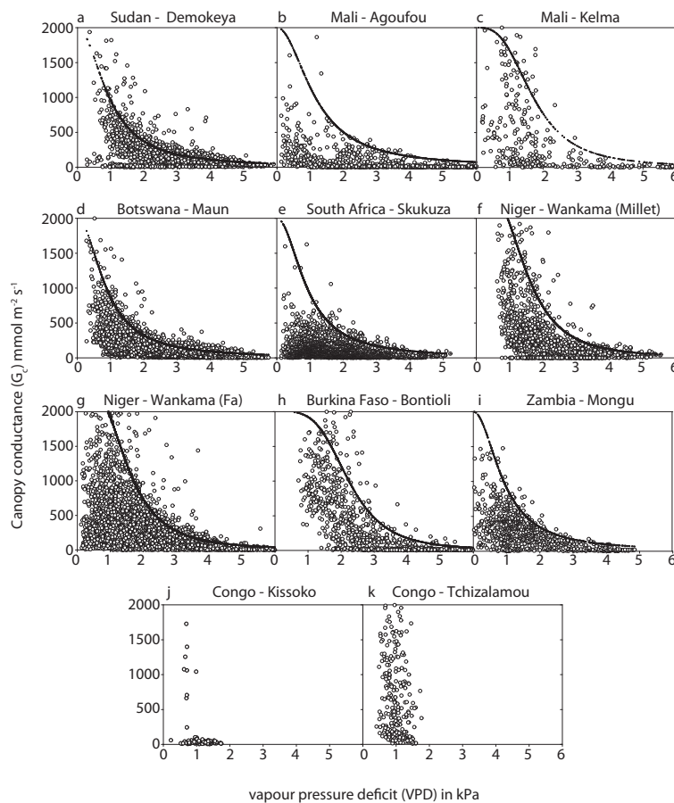
Fig. 7. The relationship between canopy conductance and VPD. Canopy conductance decreases with increasing values of VPD.
