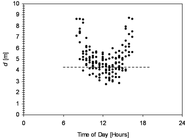
FIG. 1. Diurnal course of the displacement height as obtained from Eq. (4) (dots); horizontal line shows value of the displacement height when calculated as d = 2/3 z_{veg} .
