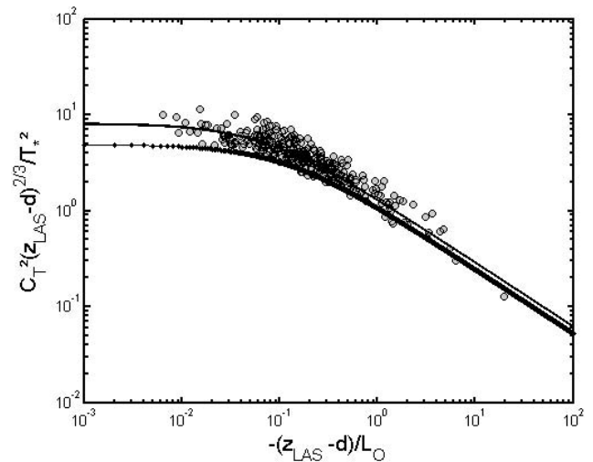
Fig. 2. Observed values of C_{T^2}(z_{\text{LAS}} - d)^{2/3}/T_*^2 plotted against observed (z_{\text{LAS}} - d)/L_O during the 3 periods. Data that diverges from MOST behavior are rejected. Solid line represents the scaling of the universal function given by Hill (1992) and dotted line represents the one by de Bruin (1993).
