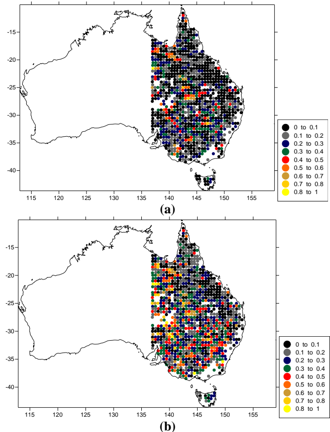
Fig. 4. Coefficient of determination ( R^2 , p < 0.05^* ) of the regression equations computed from the SMOS and MODIS data for the eastern part of Australia during to the period covering September to December (a) setting NDVI=0 and (b) accounting for the NDVI index in the regression equation. (Sept.-Dec., 2010)
