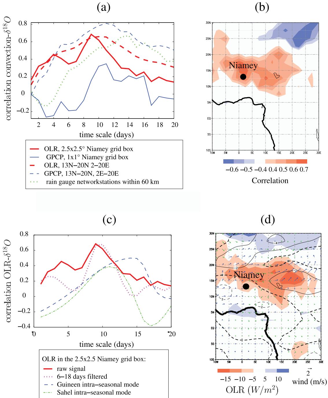
Figure 2. (a) Correlation between \delta^{18}O of organized events after the onset and different proxies of convective activity averaged over the \tau_m days preceding each rainy event, as a function of \tau_m : OLR in the 2.5 \times 2.5^\circ Niamey grid box (thick solid red), GPCP precipitation in the 1 \times 1^\circ Niamey grid box (thin solid blue), OLR (thick dashed red) and GPCP precipitation (thin dashed blue) both averaged over the 13^\circ N-20^\circ N-2^\circ E-20^\circ E domain, precipitation averaged over the AMMA rain gauge network stations within 60 km of the 3 sites barycenter (dotted green). (b) Correlation between the \delta^{18}O of the events and the OLR averaged over the 9 days preceding each event. (c) Solid red, same as heavy red line in Figure 2a; dotted magenta, same for 6–18 days filtered OLR; dashed blue and dash-dotted green, same for time series of 10–60 days filtered OLR projected on the Sahelian and Guinean modes of OLR variability [Mounier and Janicot, 2004]. (d) Difference between low \delta^{18}O and high \delta^{18}O composites, for organized events after the onset: difference of the composites of OLR averaged over the 9 previous days (shading), of 600 hPa zonal winds (contours, zero, positive and negative isolines in thick dashed, thin solid and thin dashed respectively) and of 950 hPa winds (vectors).
